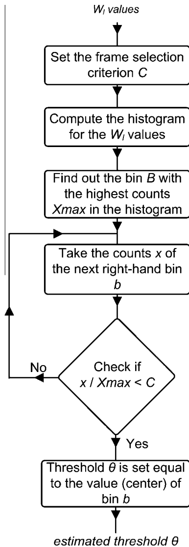
Fig. 7. The threshold estimation algorithm.
